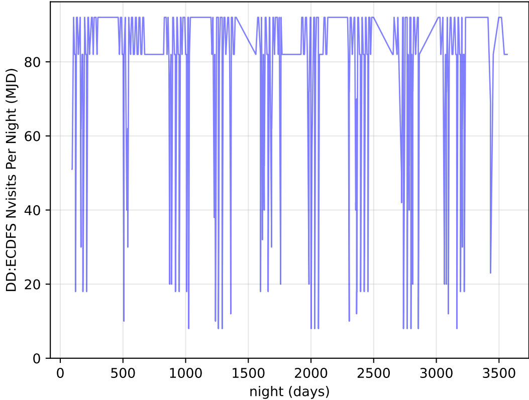
too_elab_r32_d3_ugrizy_v3.4_10yrs all bands: DD:ECDFS Nvisits Per Night
