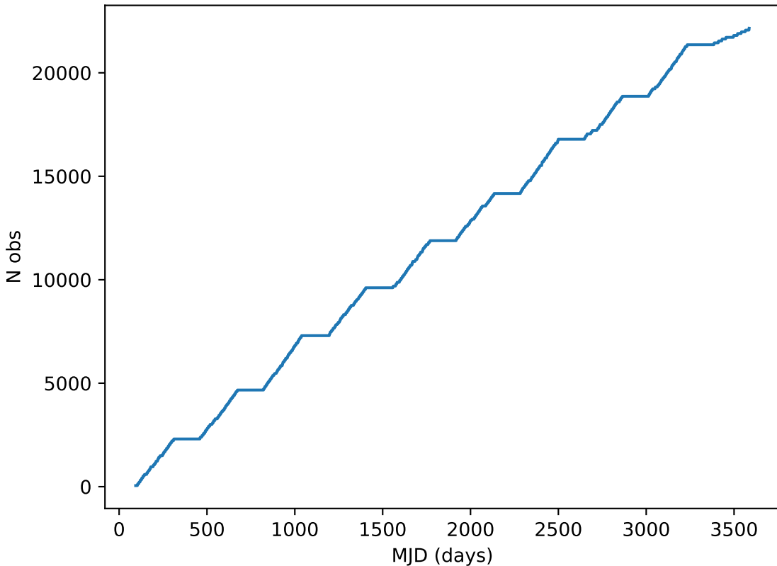
too_elab_r32_d3_ugrizy_v3.4_10yrs all bands: DD:ECDFS Cumulative NVisits
