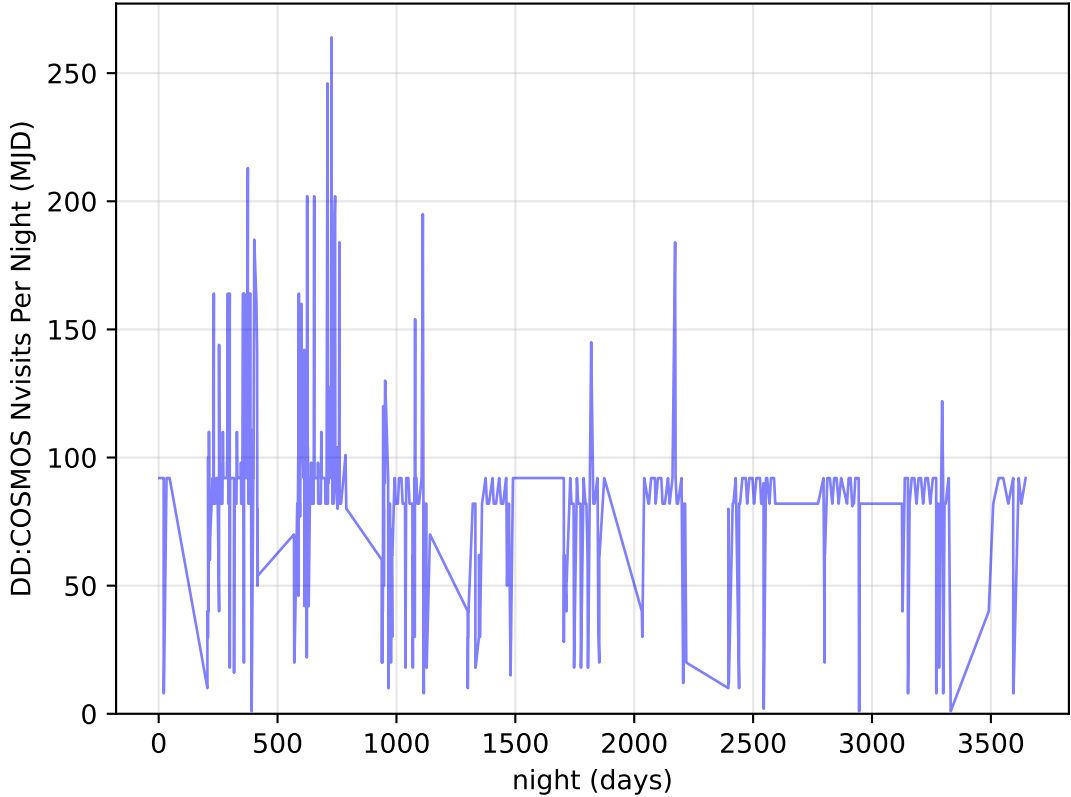
too_elab_r32_d3_ugrizy_v3.4_10yrs all bands: DD: COSMOS Nvisits Per Night
