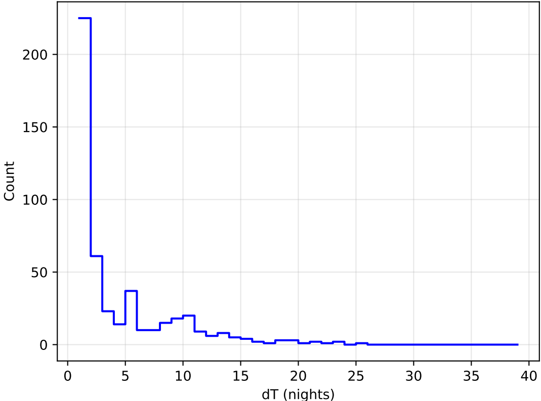
too_elab_r32_d3_ugrizy_v3.4_10yrs all bands: DD: COSMOS Delta Nights Histogram
