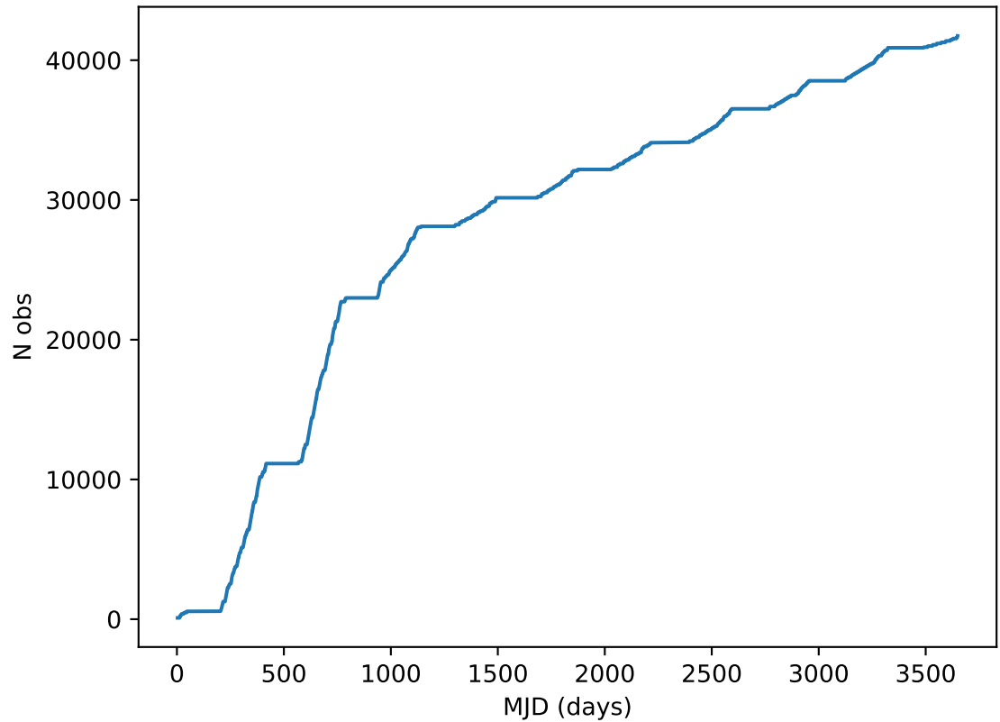
too_elab_r32_d3_ugrizy_v3.4_10yrs all bands: DD: COSMOS Cumulative NVisits
