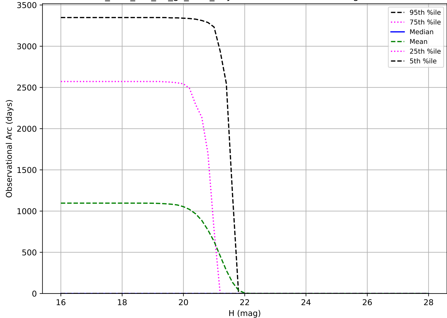
too_elab_r32_d3_gz_v3.4_10yrs: Observational Arc Length Vatira
