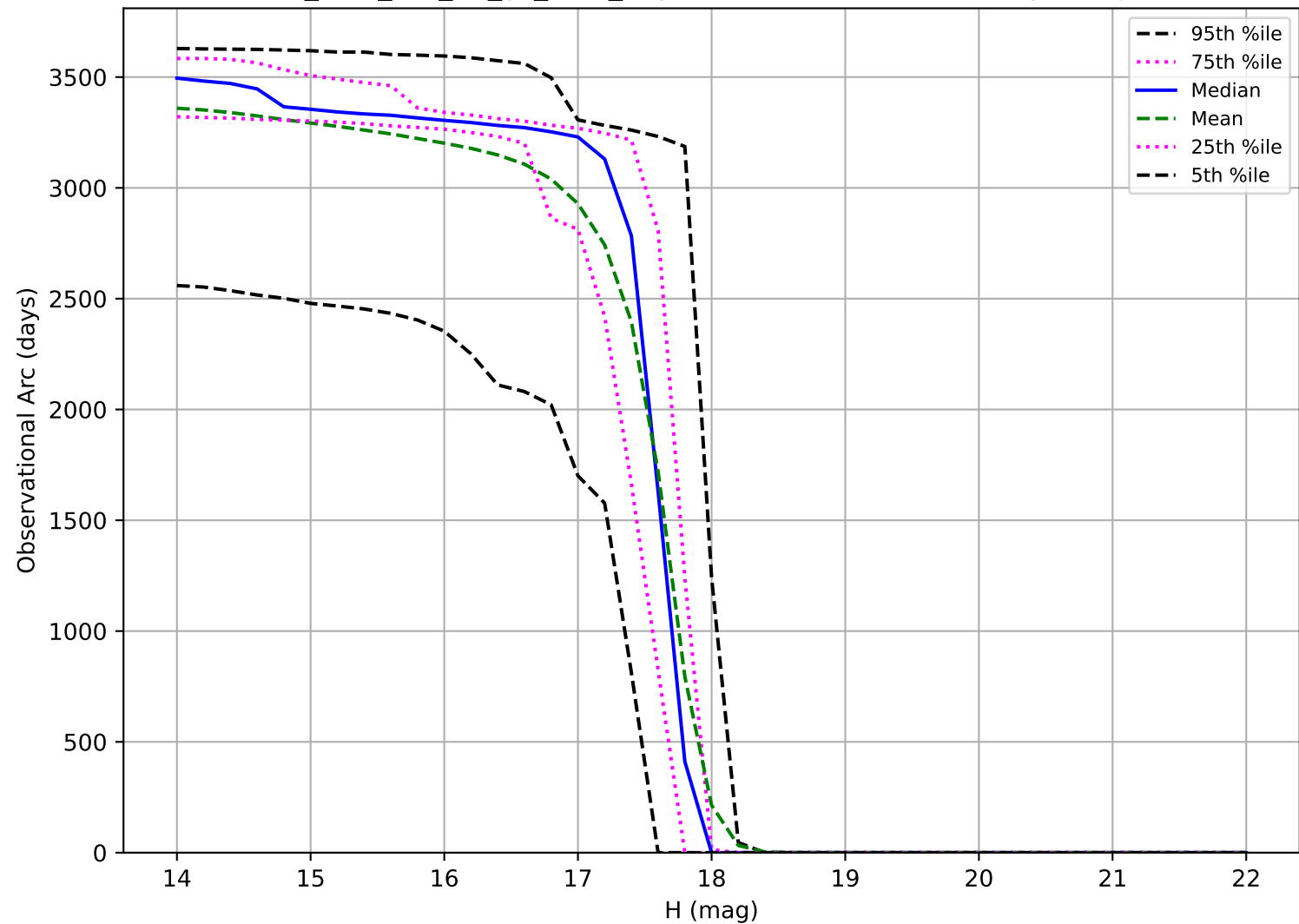
too_elab_r32_d3_gz_v3.4_10yrs: Observational Arc Length Trojan
