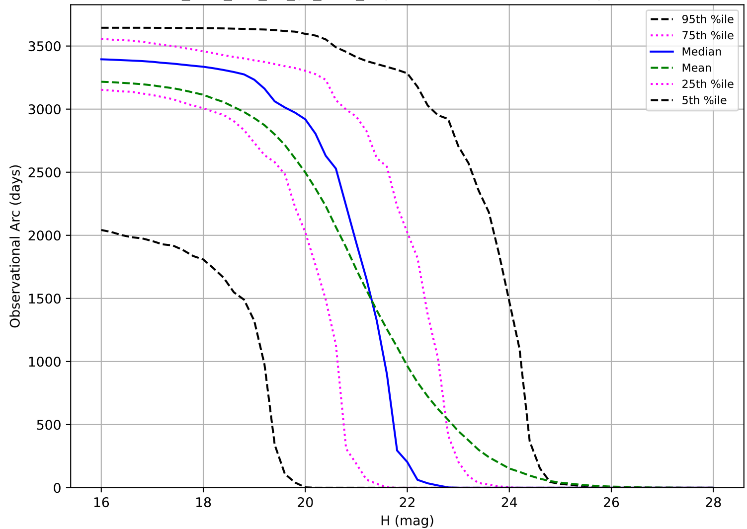
too_elab_r32_d3_gz_v3.4_10yrs: Observational Arc Length PHA
