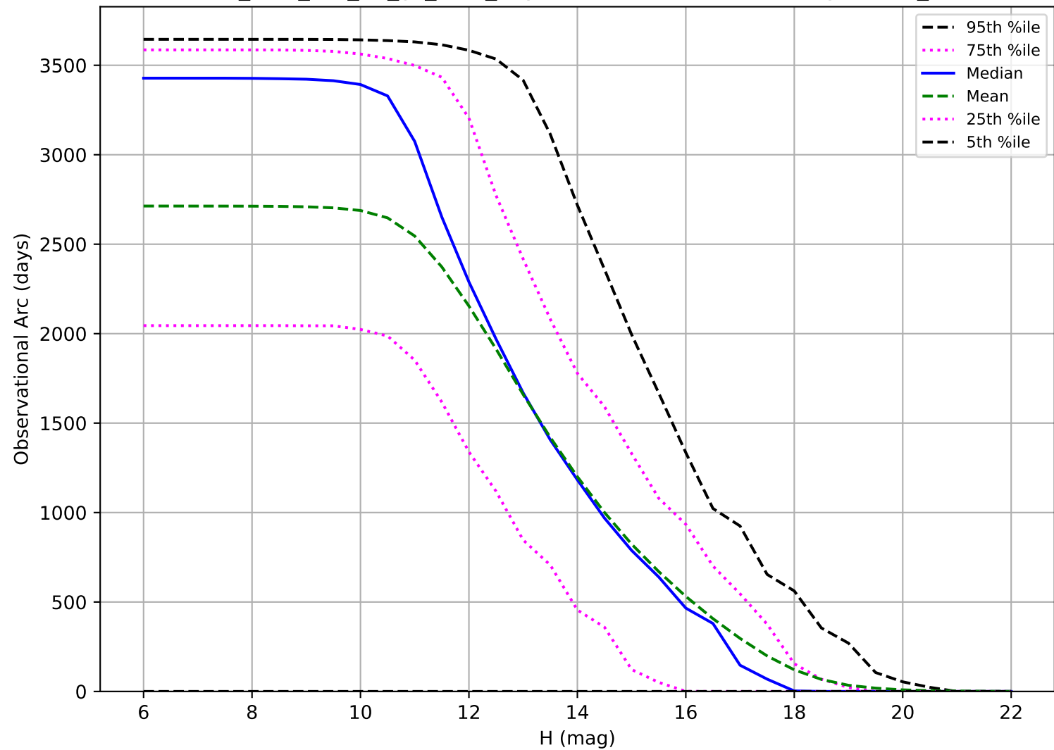
too_elab_r32_d3_gz_v3.4_10yrs: Observational Arc Length OCC_r5
