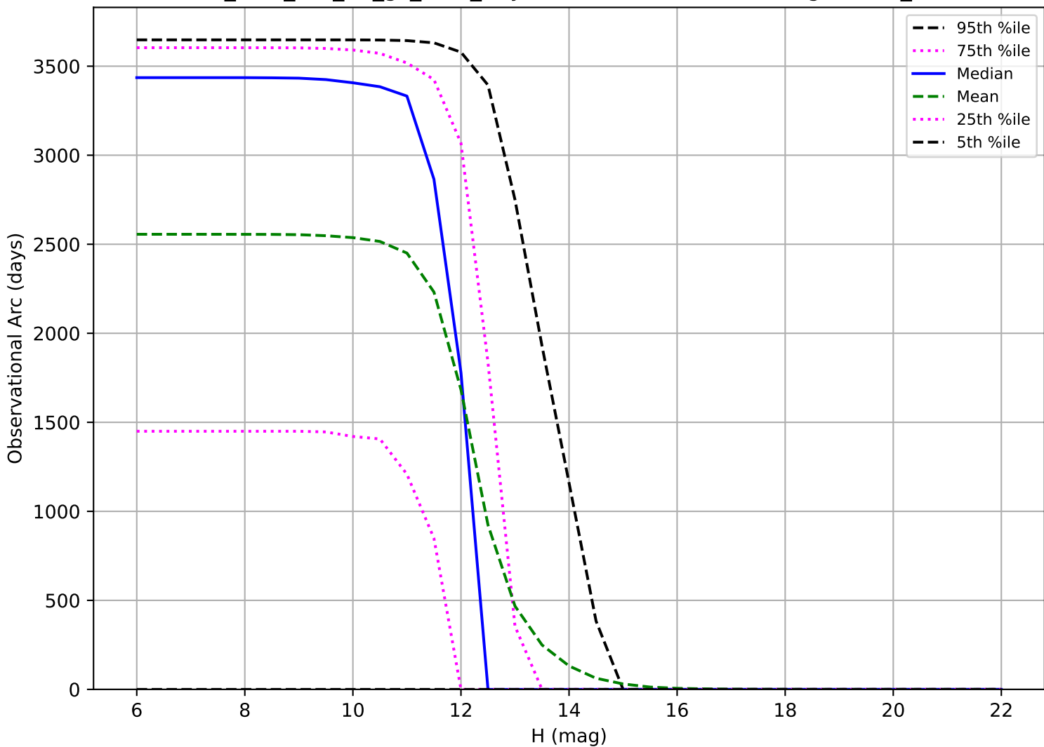
too_elab_r32_d3_gz_v3.4_10yrs: Observational Arc Length OCC_r20
