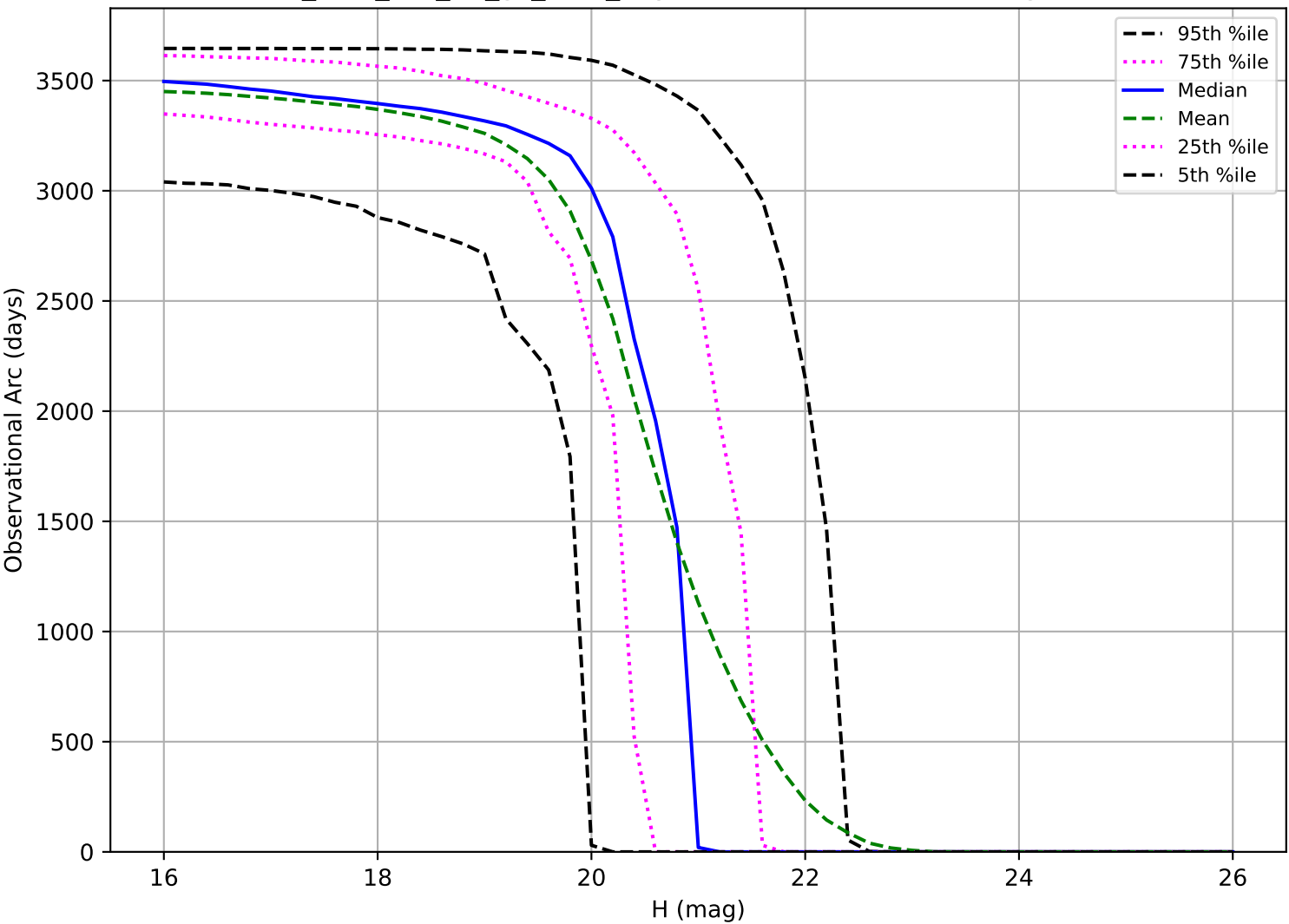
too_elab_r32_d3_gz_v3.4_10yrs: Observational Arc Length MBA
