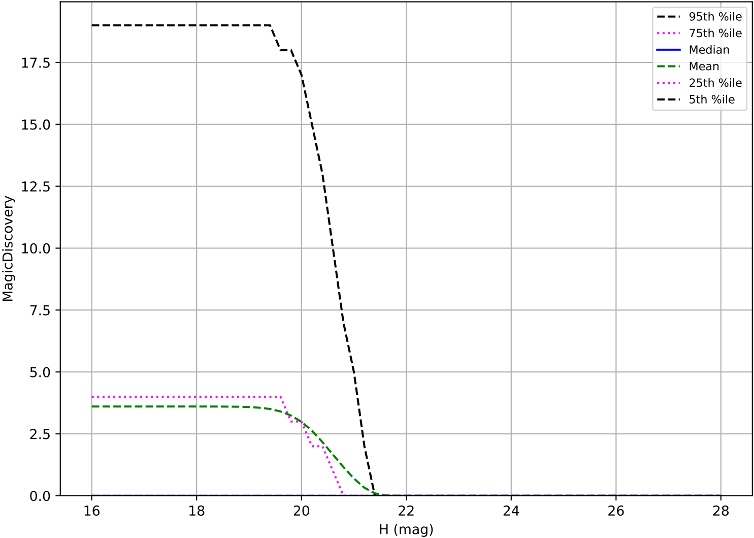
too_elab_r32_d3_gz_v3.4_10yrs: Vatira 6 detections in 60 nights detection loss
