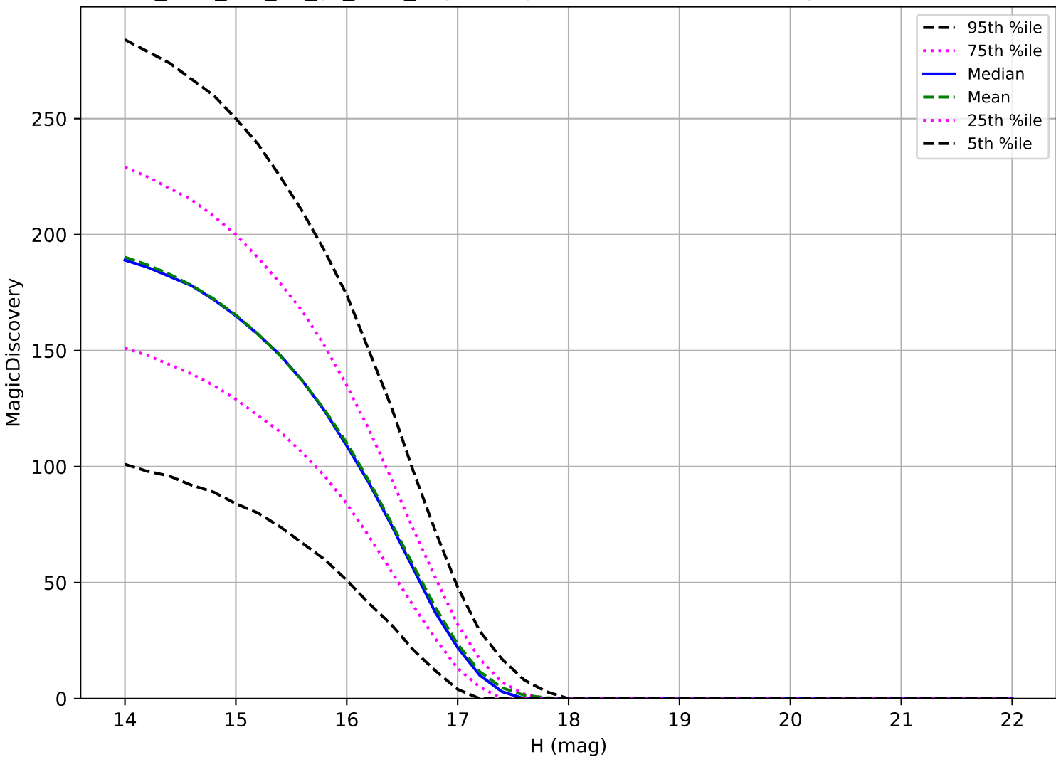
too_elab_r32_d3_gz_v3.4_10yrs: Trojan 6 detections in 60 nights detection loss
