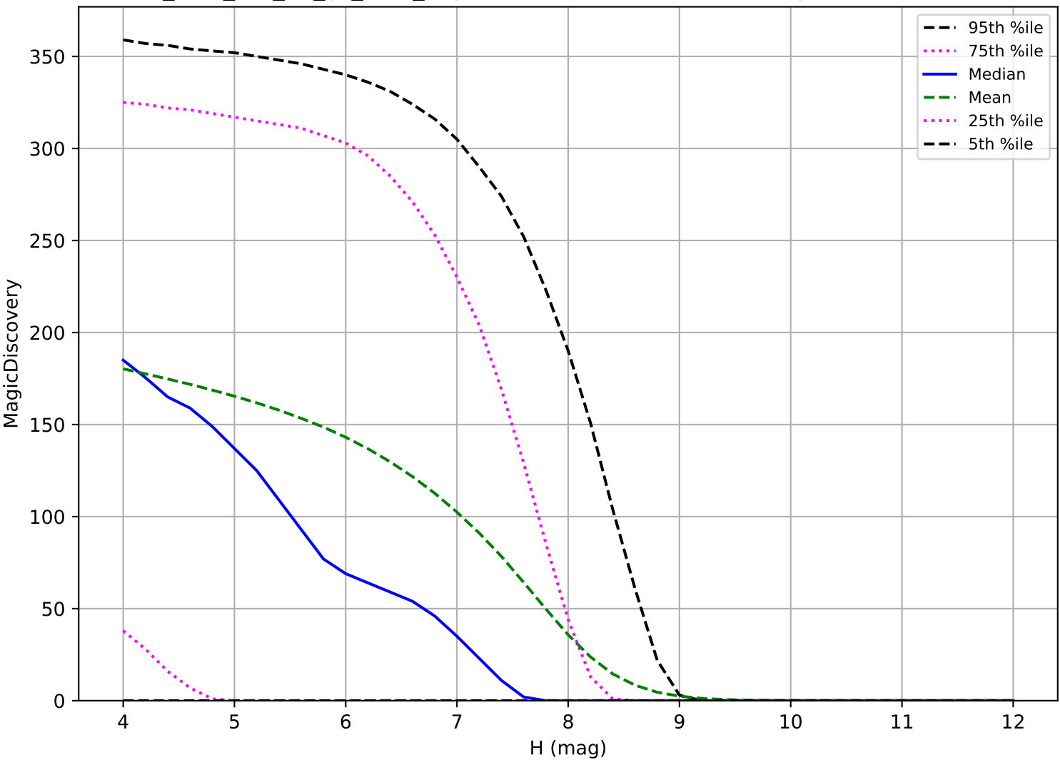
too_elab_r32_d3_gz_v3.4_10yrs: TNO 6 detections in 60 nights detection loss
