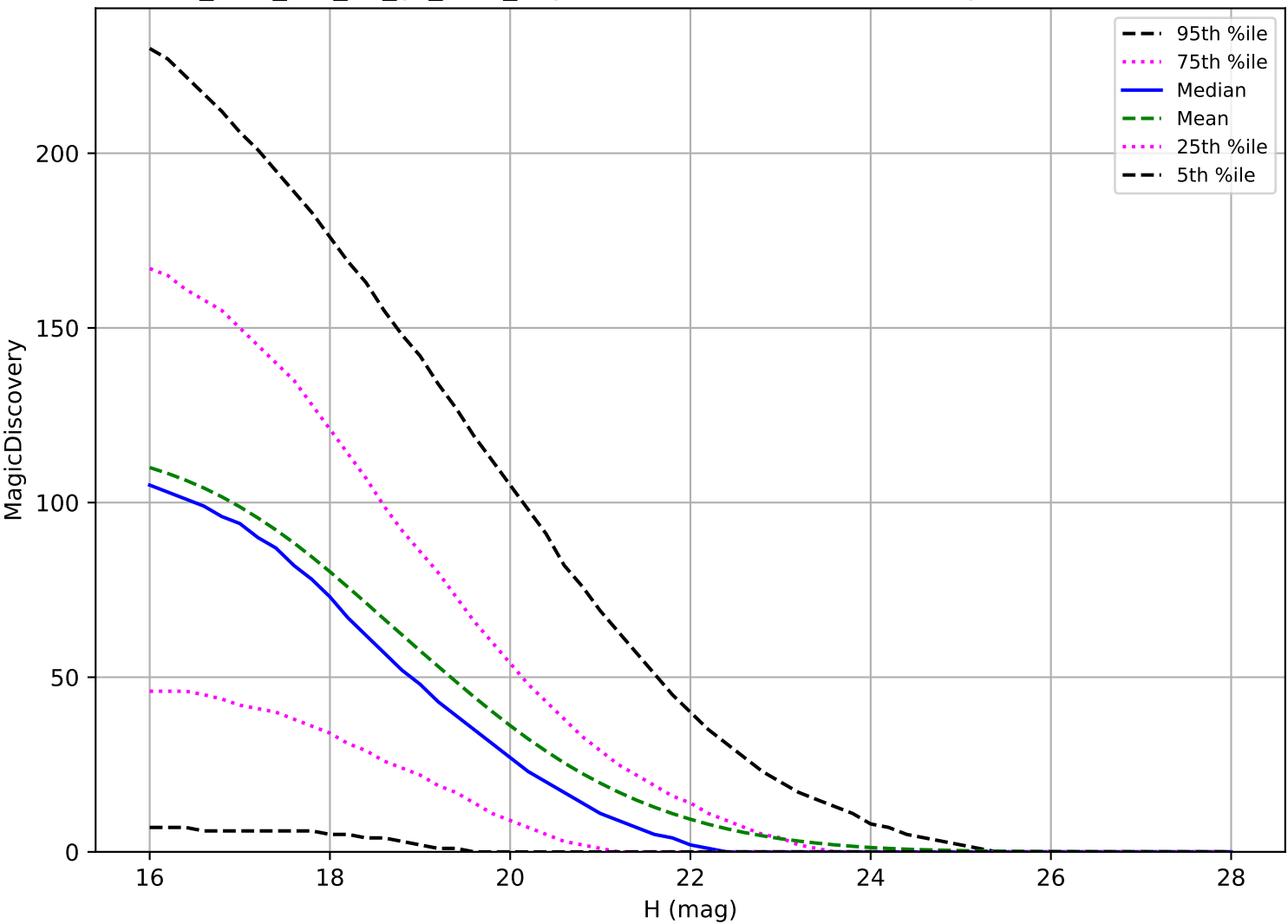
too_elab_r32_d3_gz_v3.4_10yrs: PHA 6 detections in 60 nights detection loss
