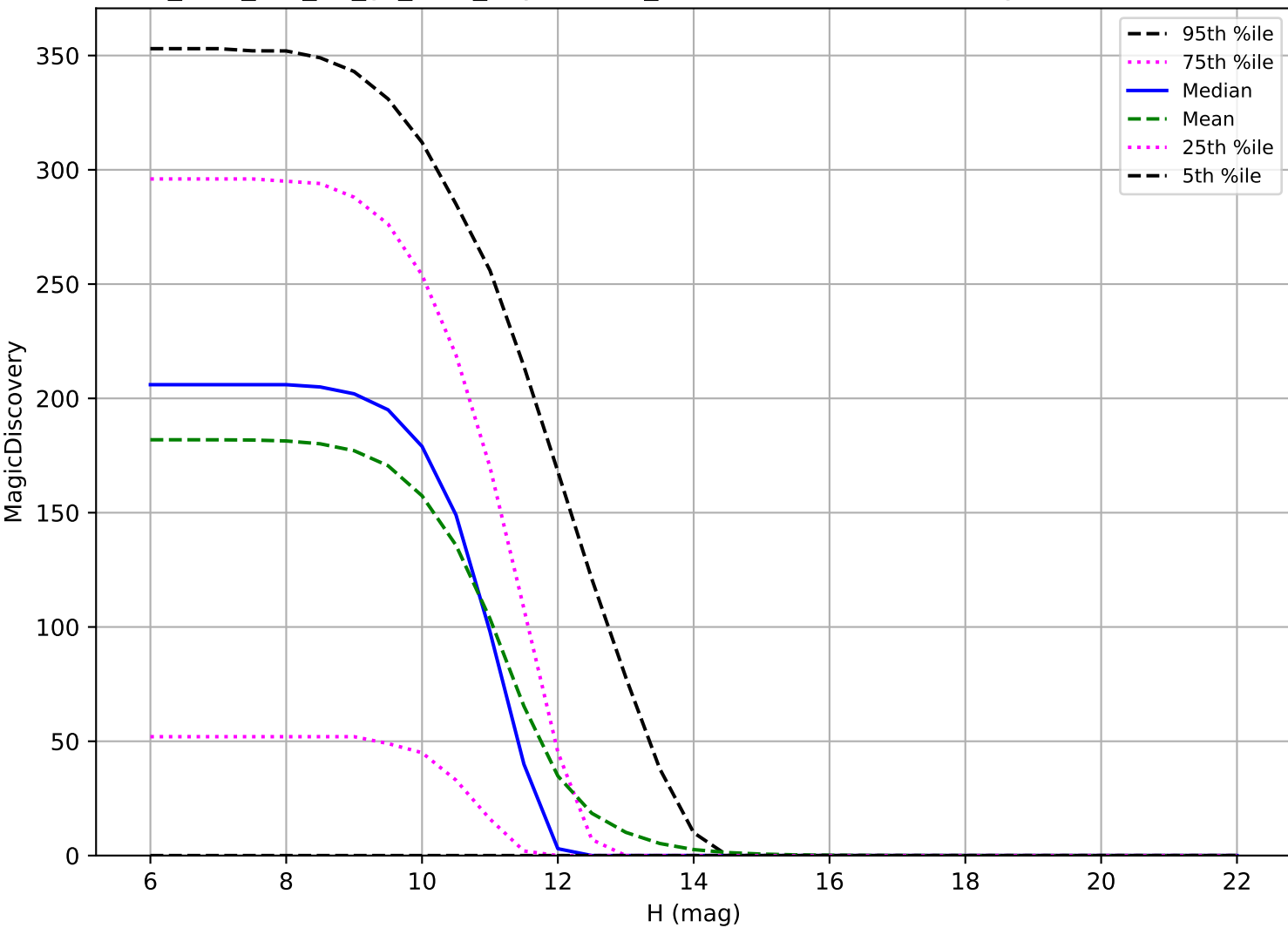
too_elab_r32_d3_gz_v3.4_10yrs: OCC_r20 6 detections in 60 nights detection loss
