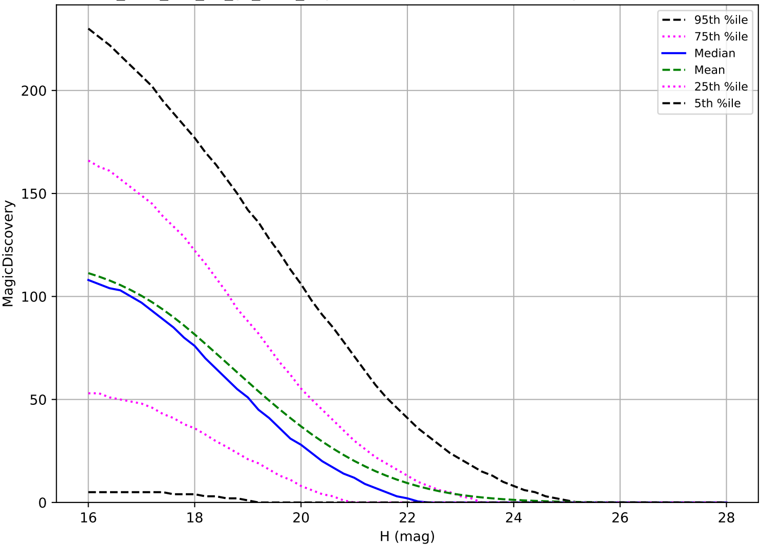
too_elab_r32_d3_gz_v3.4_10yrs: NEO 6 detections in 60 nights detection loss
