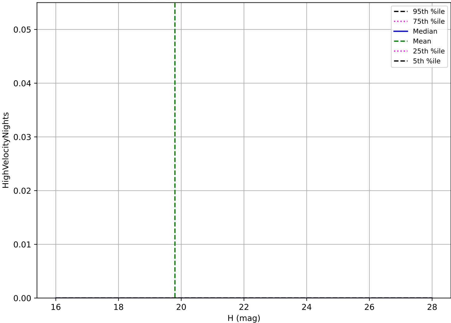
too_elab_r32_d3_gz_v3.4_10yrs: Vatira High velocity pair detection loss
