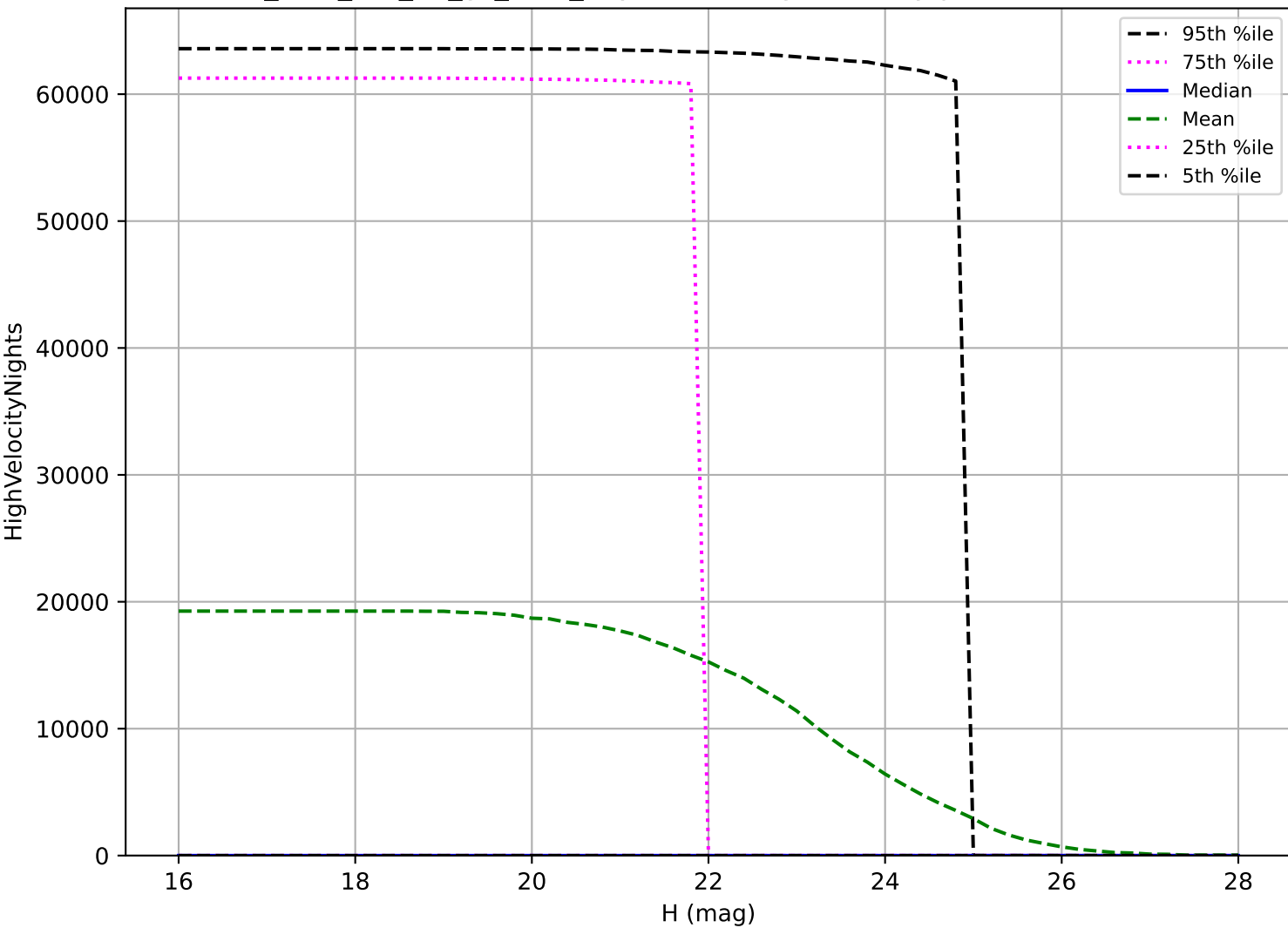
too_elab_r32_d3_gz_v3.4_10yrs: NEO High velocity pair detection loss
