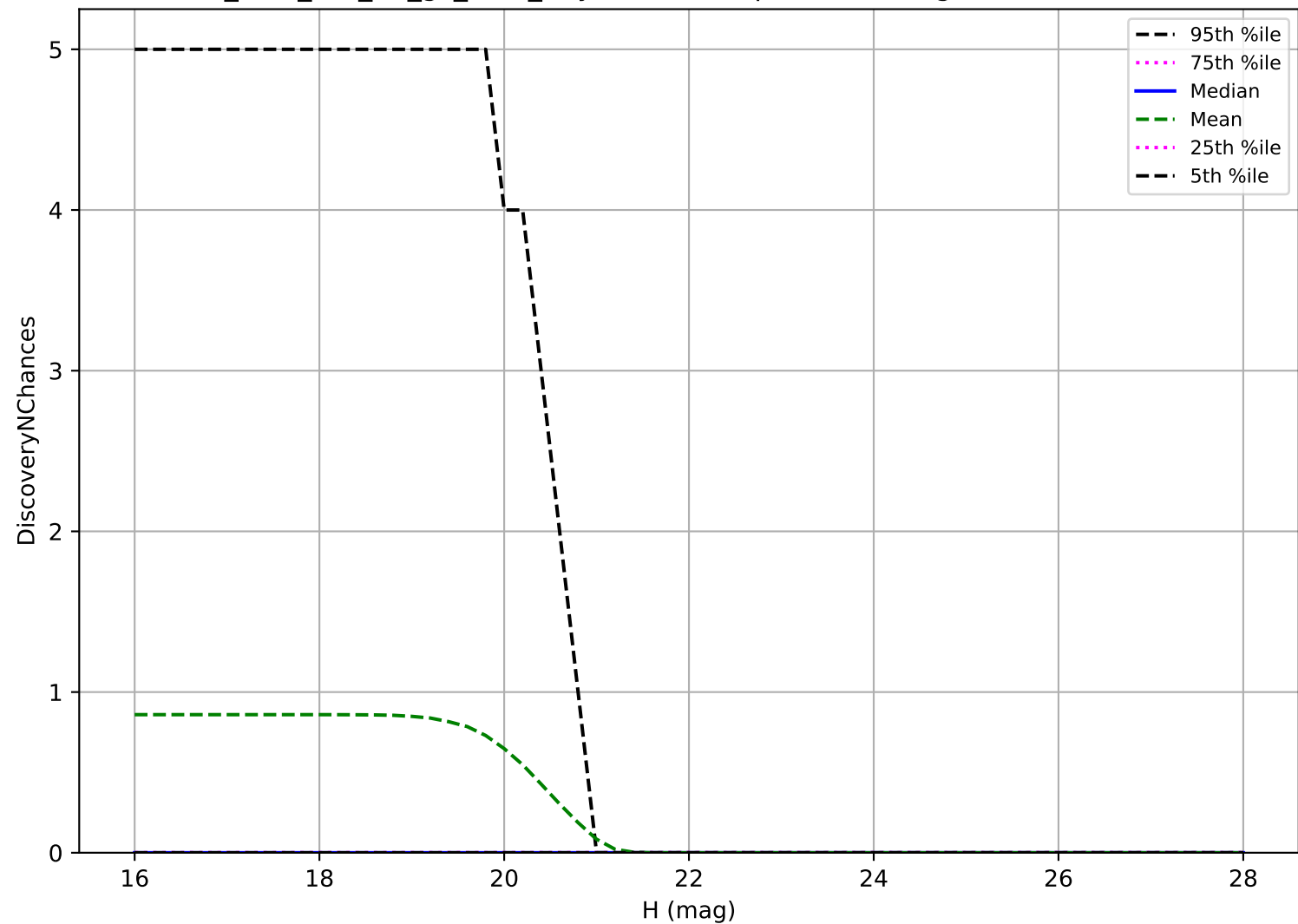
too_elab_r32_d3_gz_v3.4_10yrs: Vatira 3 pairs in 15 nights detection loss
