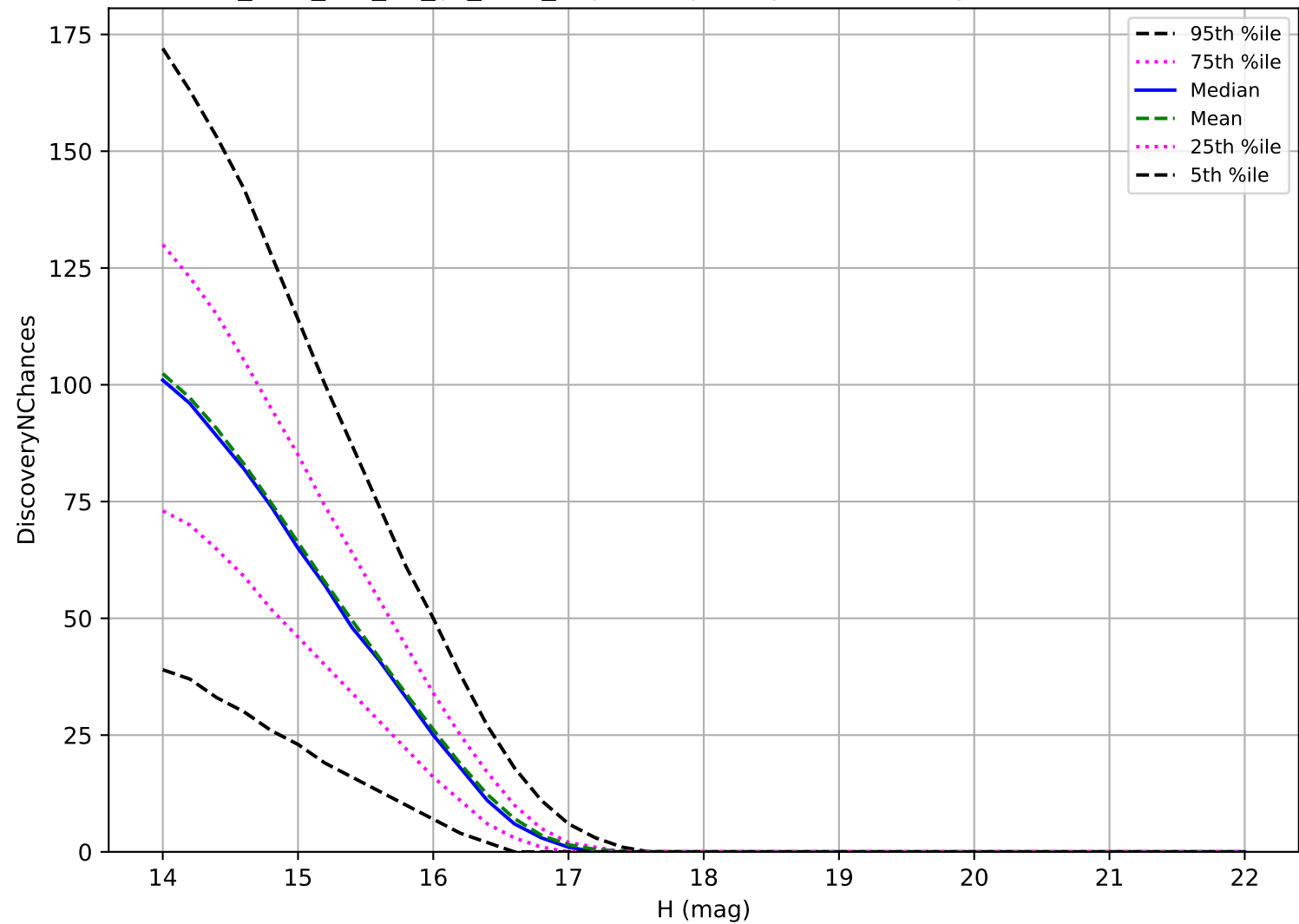
too_elab_r32_d3_gz_v3.4_10yrs: Trojan 3 pairs in 15 nights detection loss
