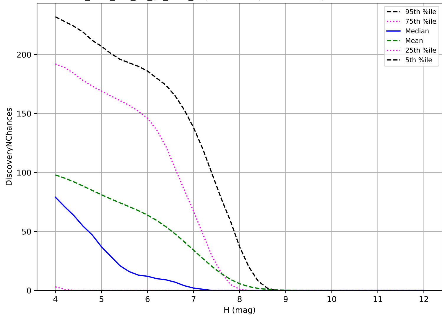
too_elab_r32_d3_gz_v3.4_10yrs: TNO 3 pairs in 15 nights detection loss
