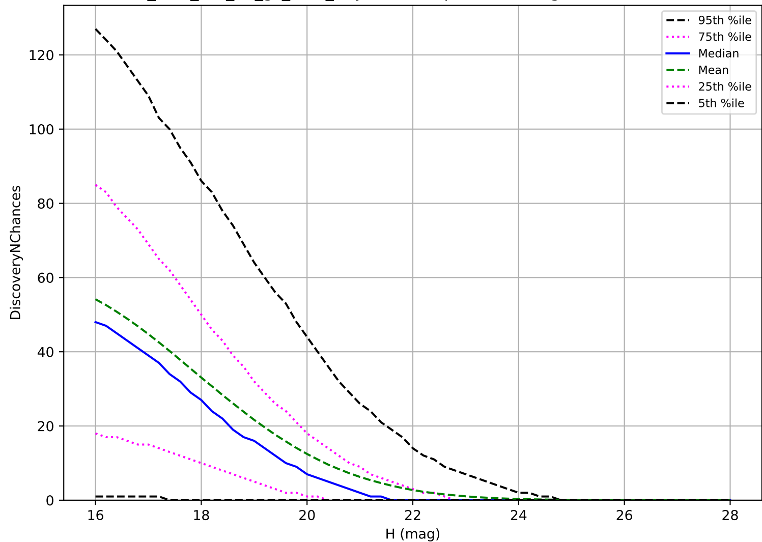
too_elab_r32_d3_gz_v3.4_10yrs: PHA 3 pairs in 15 nights detection loss
