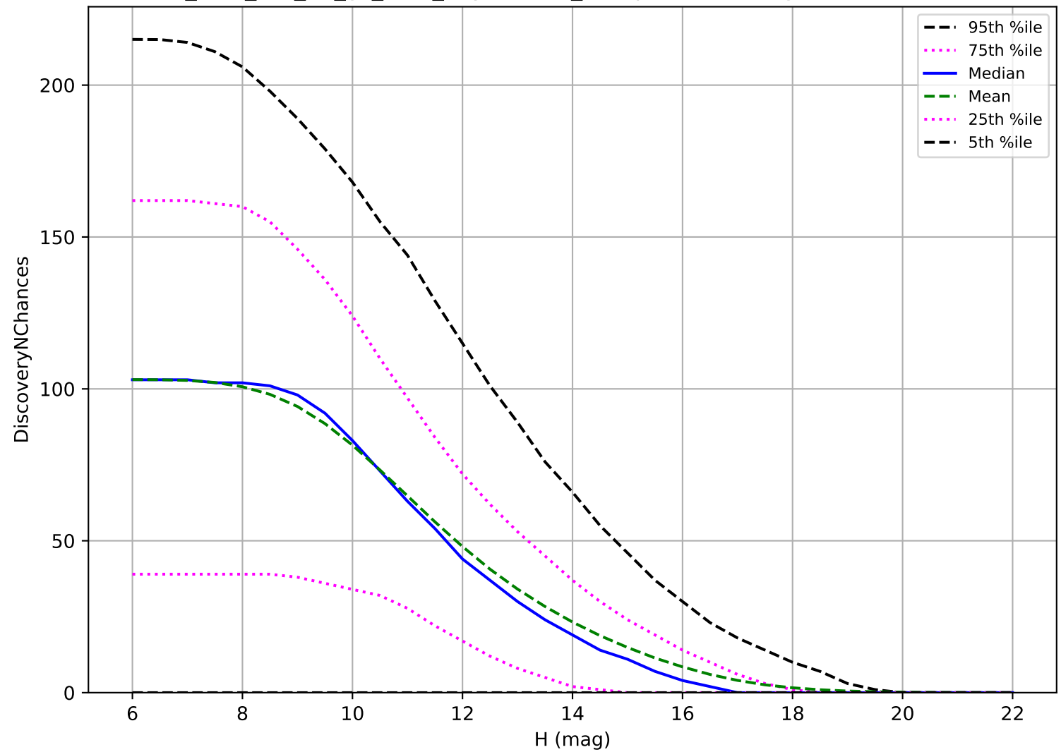
too_elab_r32_d3_gz_v3.4_10yrs: OCC_r5 3 pairs in 15 nights detection loss
