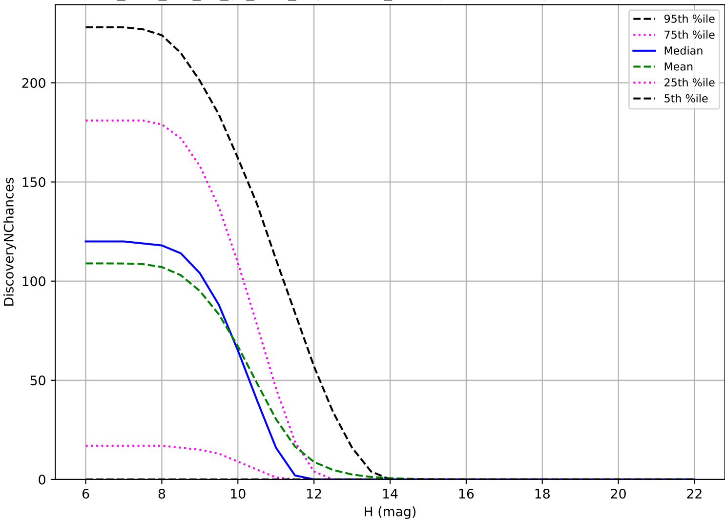
too_elab_r32_d3_gz_v3.4_10yrs: OCC_r20 3 pairs in 15 nights detection loss
