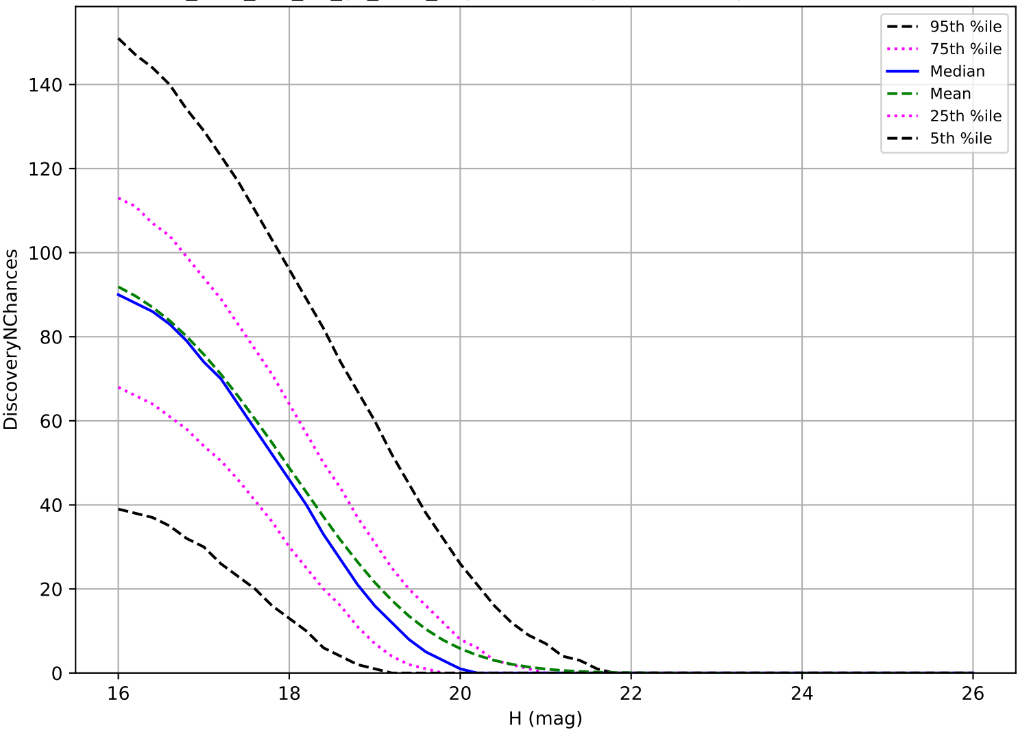
too_elab_r32_d3_gz_v3.4_10yrs: MBA 3 pairs in 15 nights detection loss
