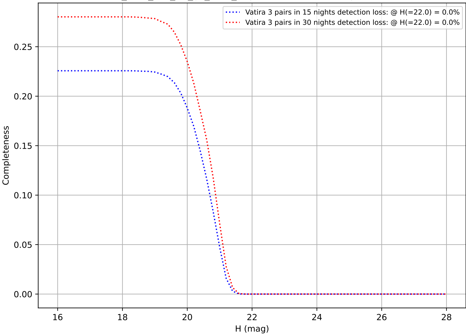
too_elab_r32_d3_gz_v3.4_10yrs: DifferentialCompleteness
