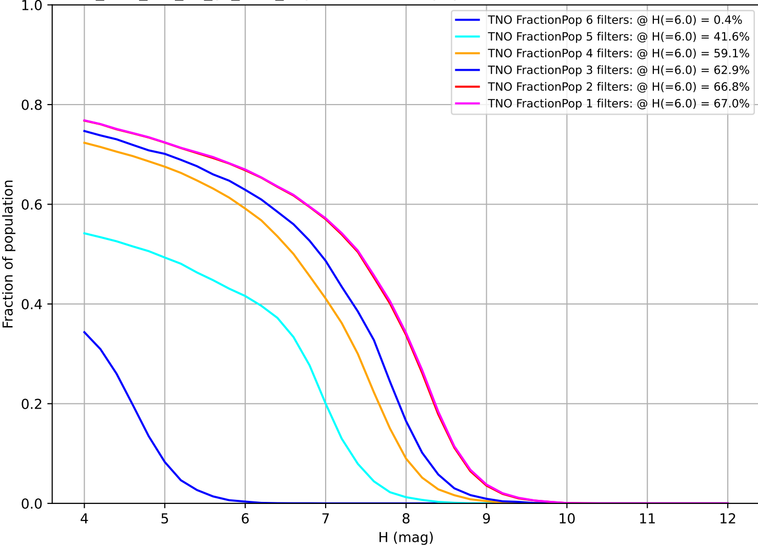
too_elab_r32_d3_gz_v3.4_10yrs: Fraction of population with colors in X filters TNO
