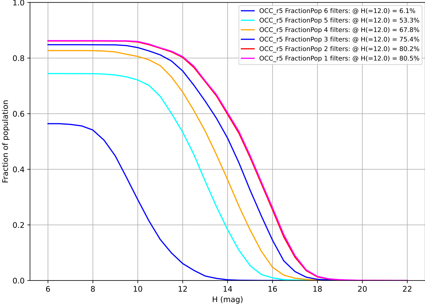
too_elab_r32_d3_gz_v3.4_10yrs: Fraction of population with colors in X filters OCC_r5
