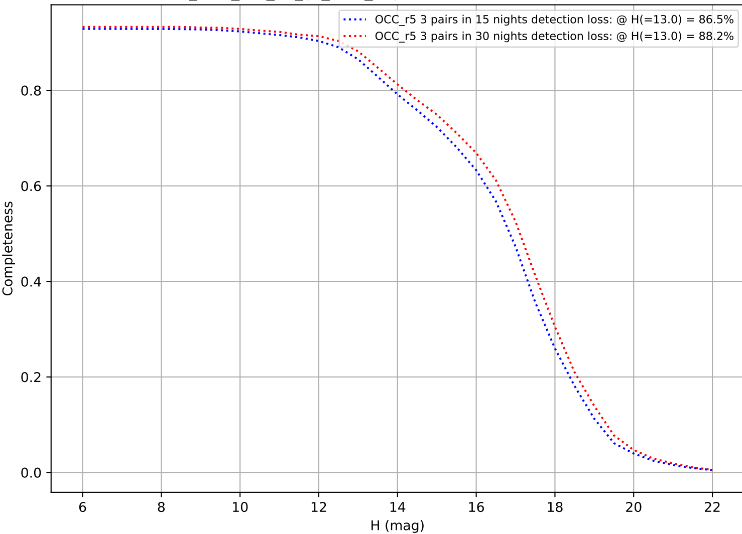
too_elab_r32_d3_gz_v3.4_10yrs: DifferentialCompleteness
