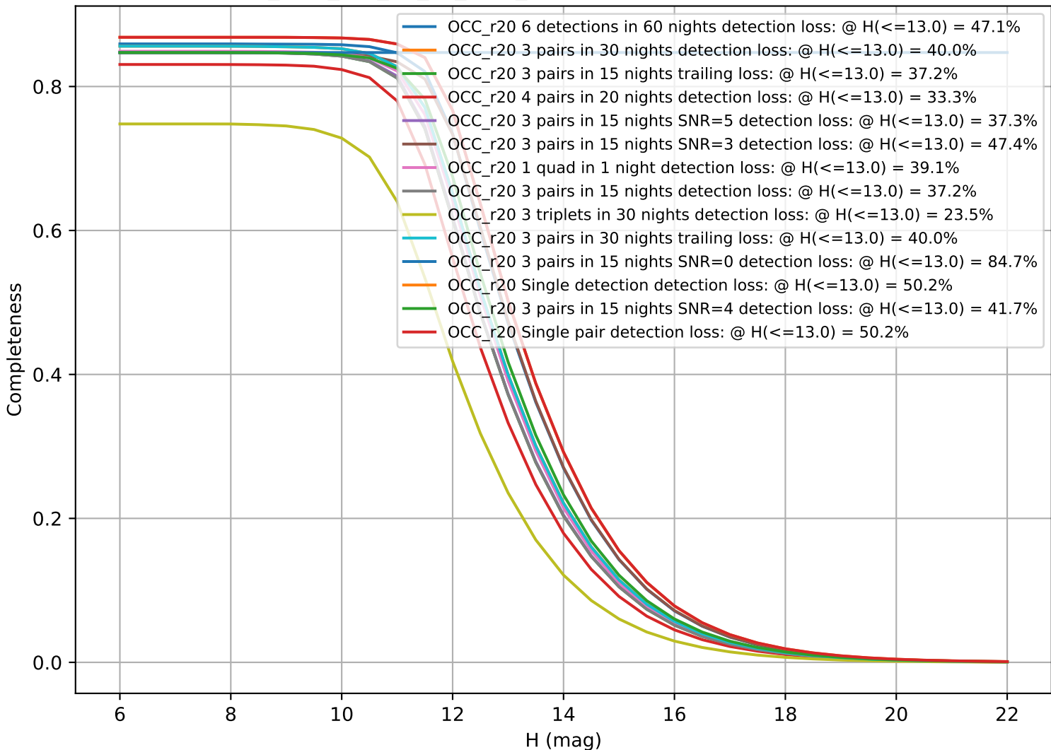
too_elab_r32_d3_gz_v3.4_10yrs: CumulativeCompleteness
