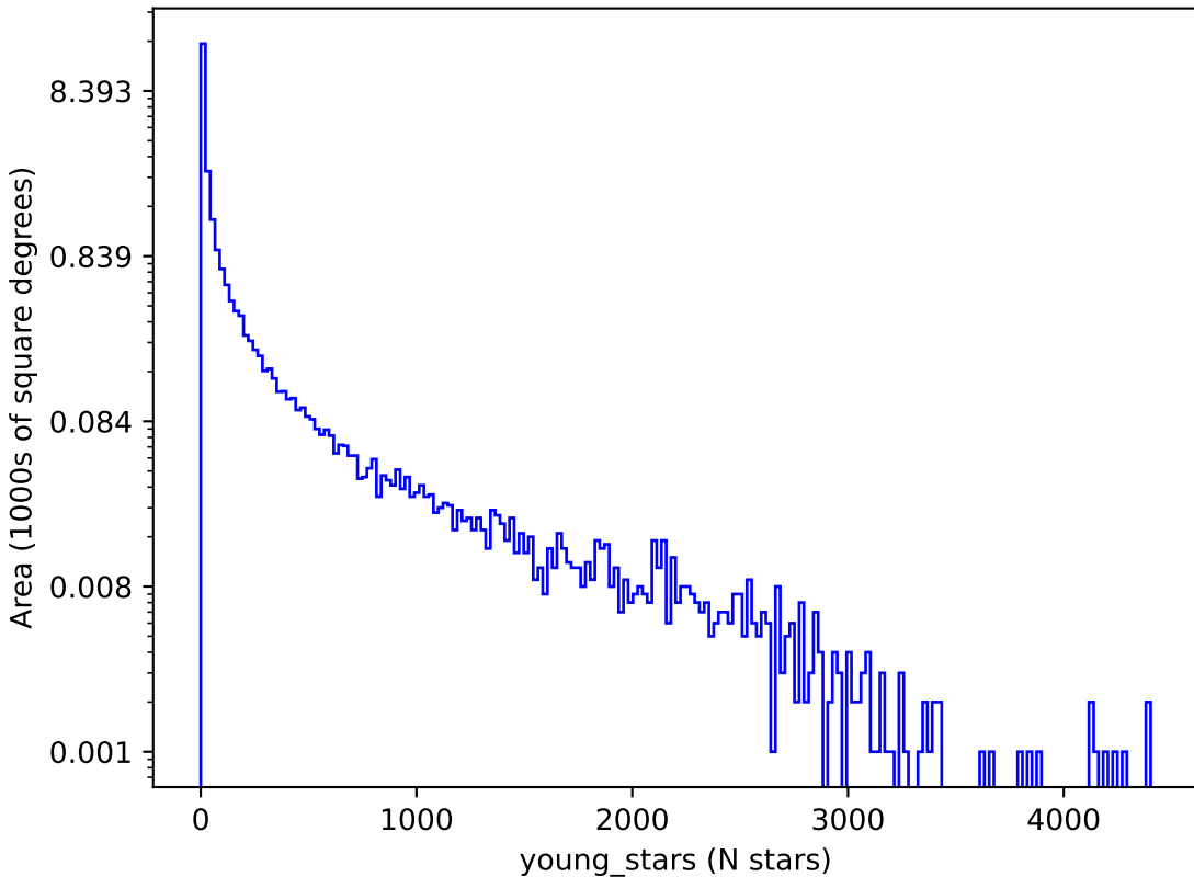
too_elab_r32_d3_gz_v3.4_10yrs : young_stars
