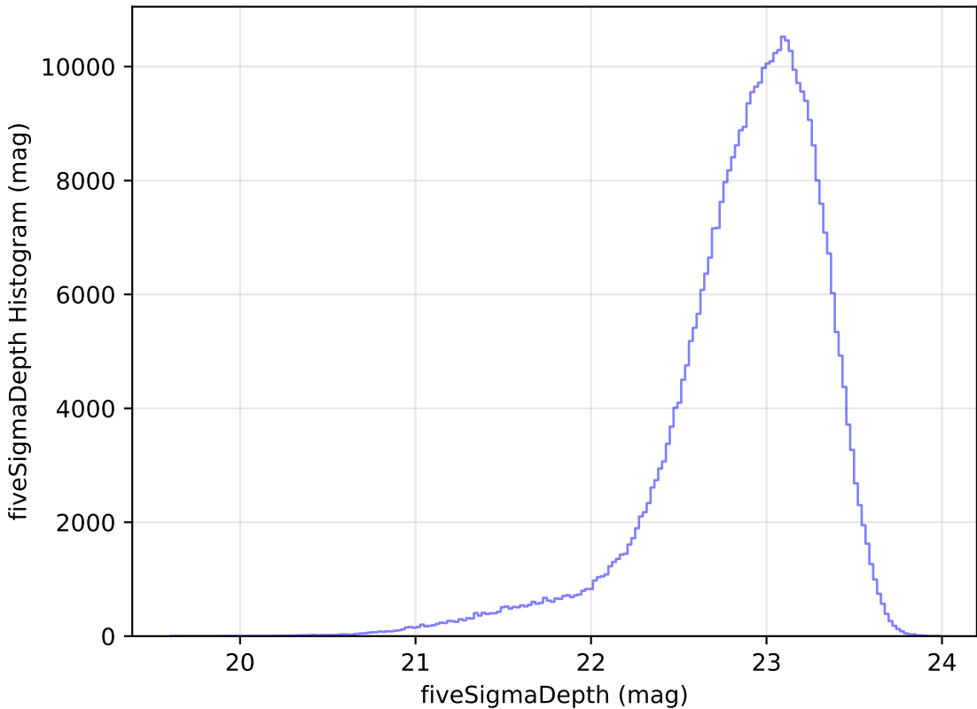
too_elab_r32_d3_gz_v3.4_10yrs z: fiveSigmaDepth Histogram
