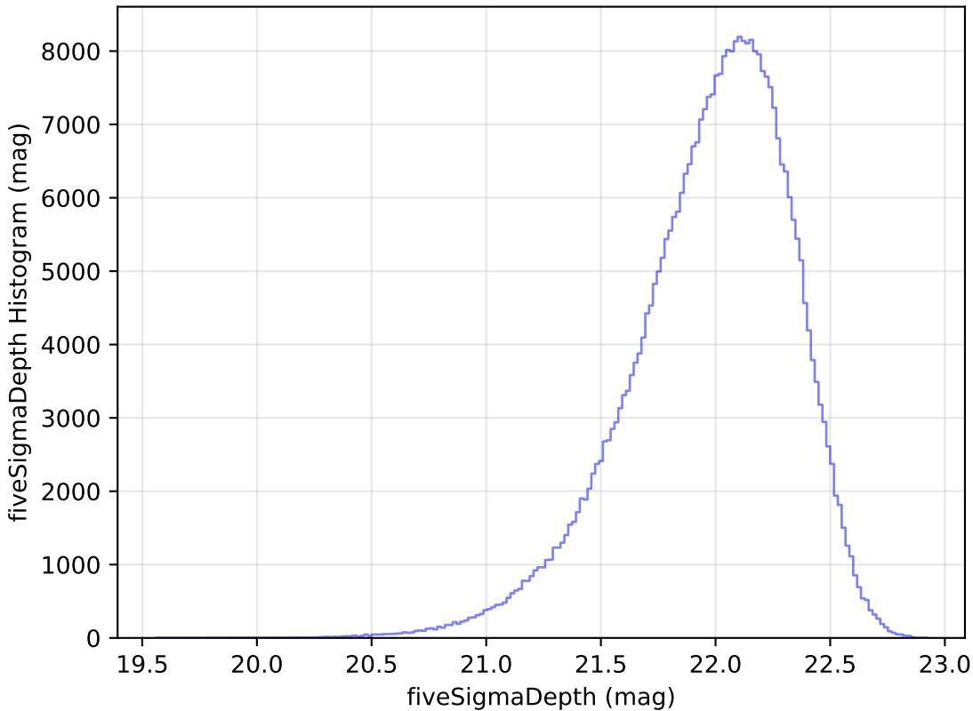
too_elab_r32_d3_gz_v3.4_10yrs y: fiveSigmaDepth Histogram
