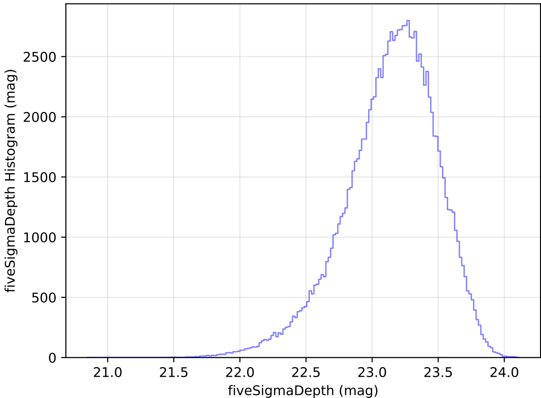
too_elab_r32_d3_gz_v3.4_10yrs u: fiveSigmaDepth Histogram
