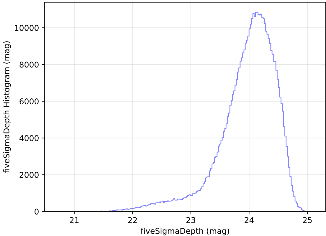
too_elab_r32_d3_gz_v3.4_10yrs r: fiveSigmaDepth Histogram
