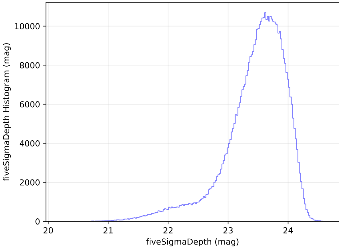
too_elab_r32_d3_gz_v3.4_10yrs i: fiveSigmaDepth Histogram
