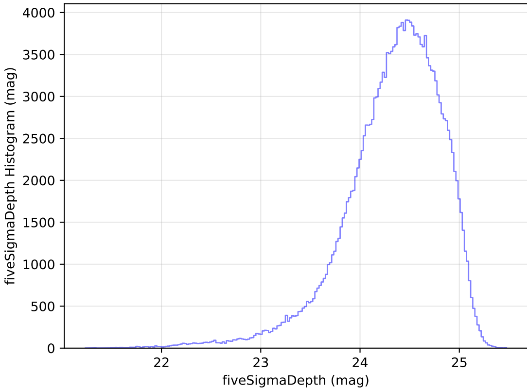
too_elab_r32_d3_gz_v3.4_10yrs g: fiveSigmaDepth Histogram
