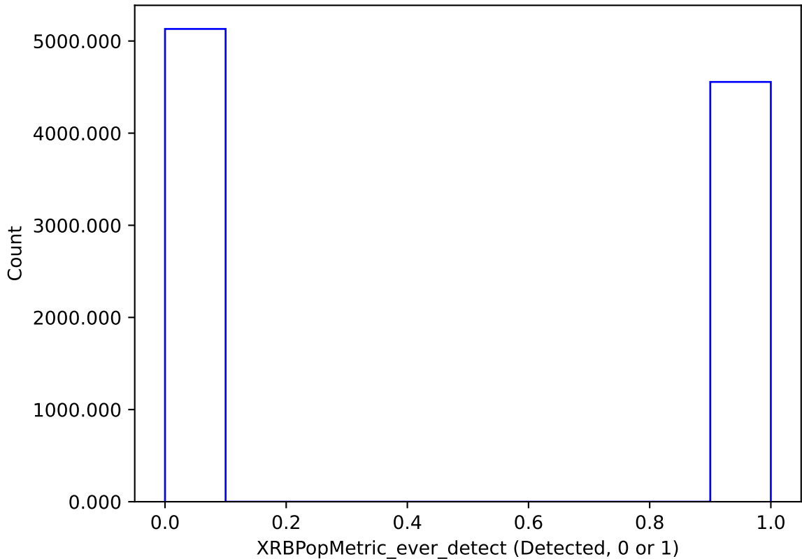
too_elab_r32_d3_gz_v3.4_10yrs : XRBPoMetric_ever_detect
