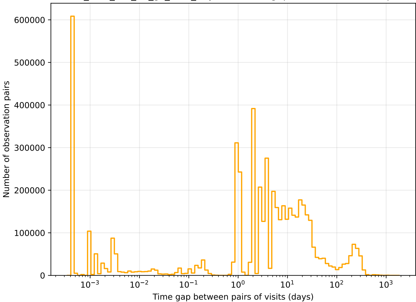
too_elab_r32_d3_gz_v3.4_10yrs r band: Tgaps observationStartMJD
