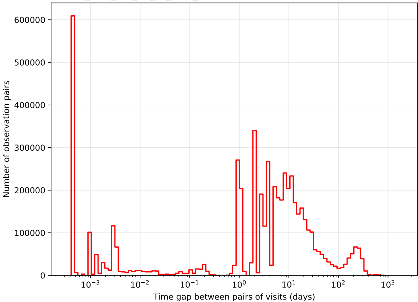
too_elab_r32_d3_gz_v3.4_10yrs i band: Tgaps observationStartMJD
