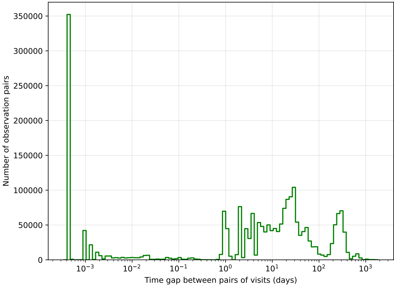
too_elab_r32_d3_gz_v3.4_10yrs g band: Tgaps observationStartMJD
