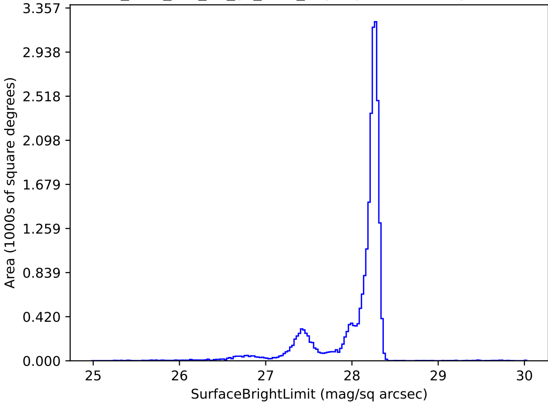
too_elab_r32_d3_gz_v3.4_10yrs y: SurfaceBrightLimit
