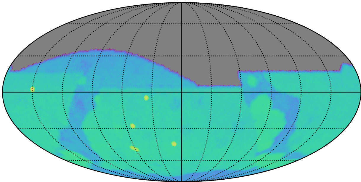
too_elab_r32_d3_gz_v3.4_10yrs g: SurfaceBrightLimit
