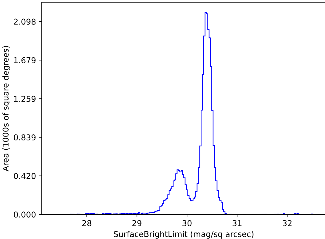
too_elab_r32_d3_gz_v3.4_10yrs g: SurfaceBrightLimit
