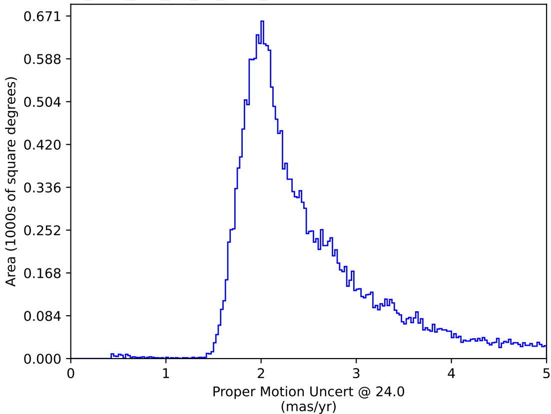
too_elab_r32_d3_gz_v3.4_10yrs : Proper Motion Uncert @ 24.0
