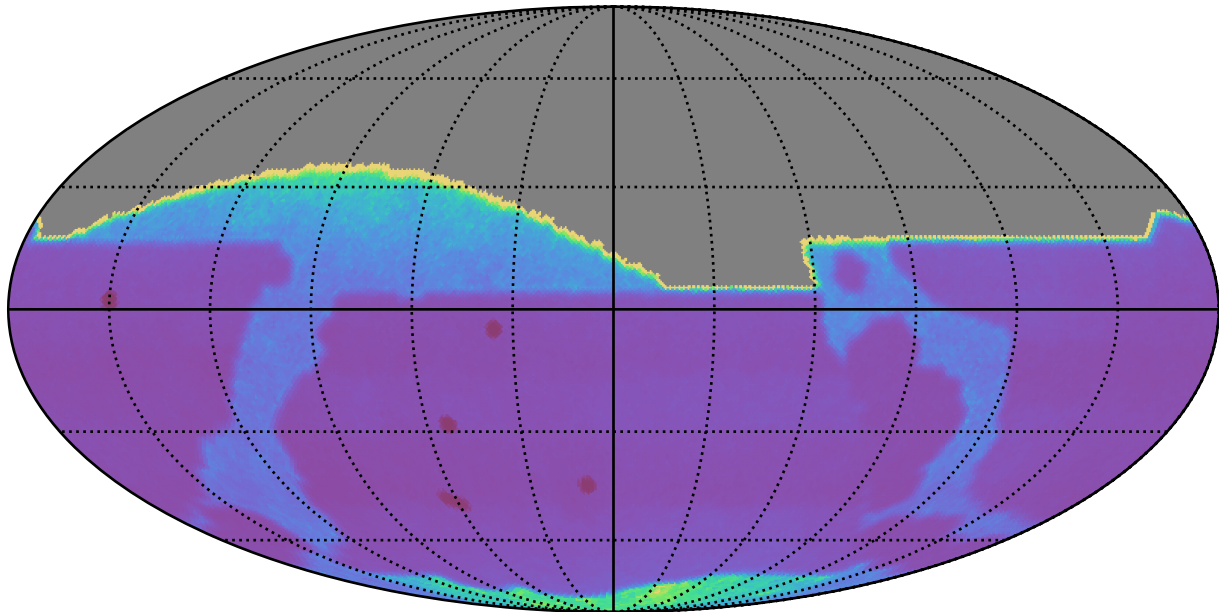
too_elab_r32_d3_gz_v3.4_10yrs : Proper Motion Uncert @ 20.5
