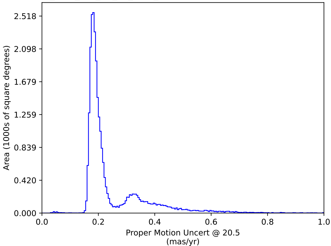
too_elab_r32_d3_gz_v3.4_10yrs : Proper Motion Uncert @ 20.5
