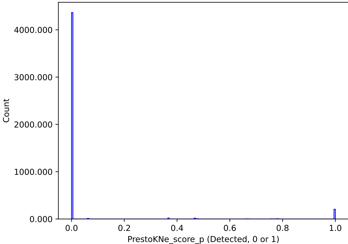
too_elab_r32_d3_gz_v3.4_10yrs : PrestoKNe_score_p
