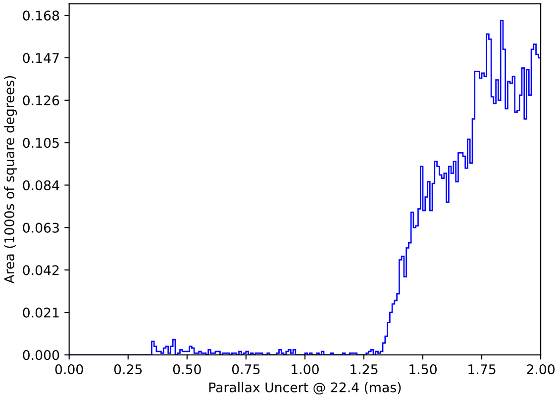
too_elab_r32_d3_gz_v3.4_10yrs : Parallax Uncert @ 22.4
